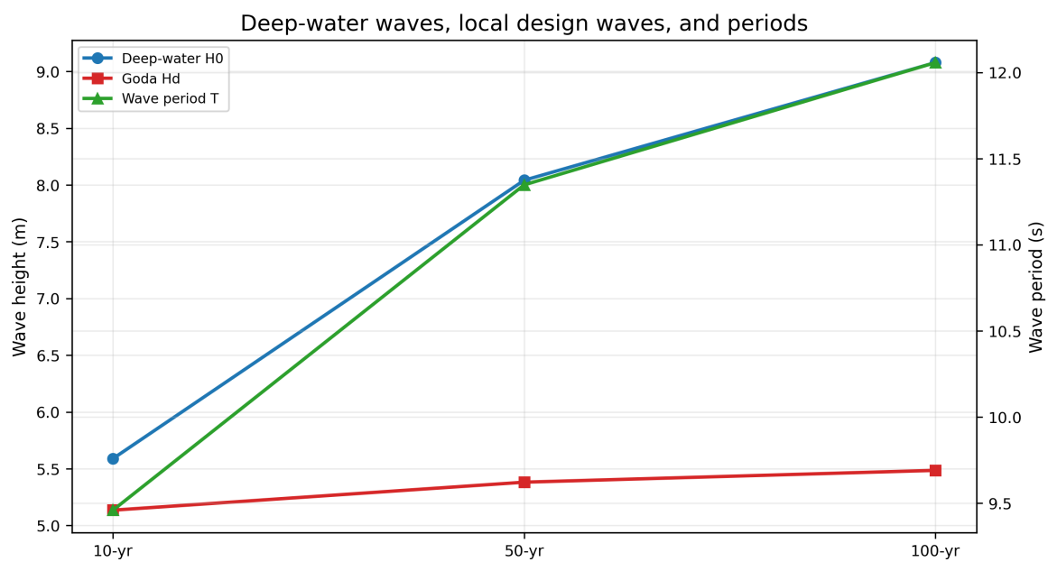
Figure 7: Comparison of deep-water wave height, local design wave height, and wave period.
