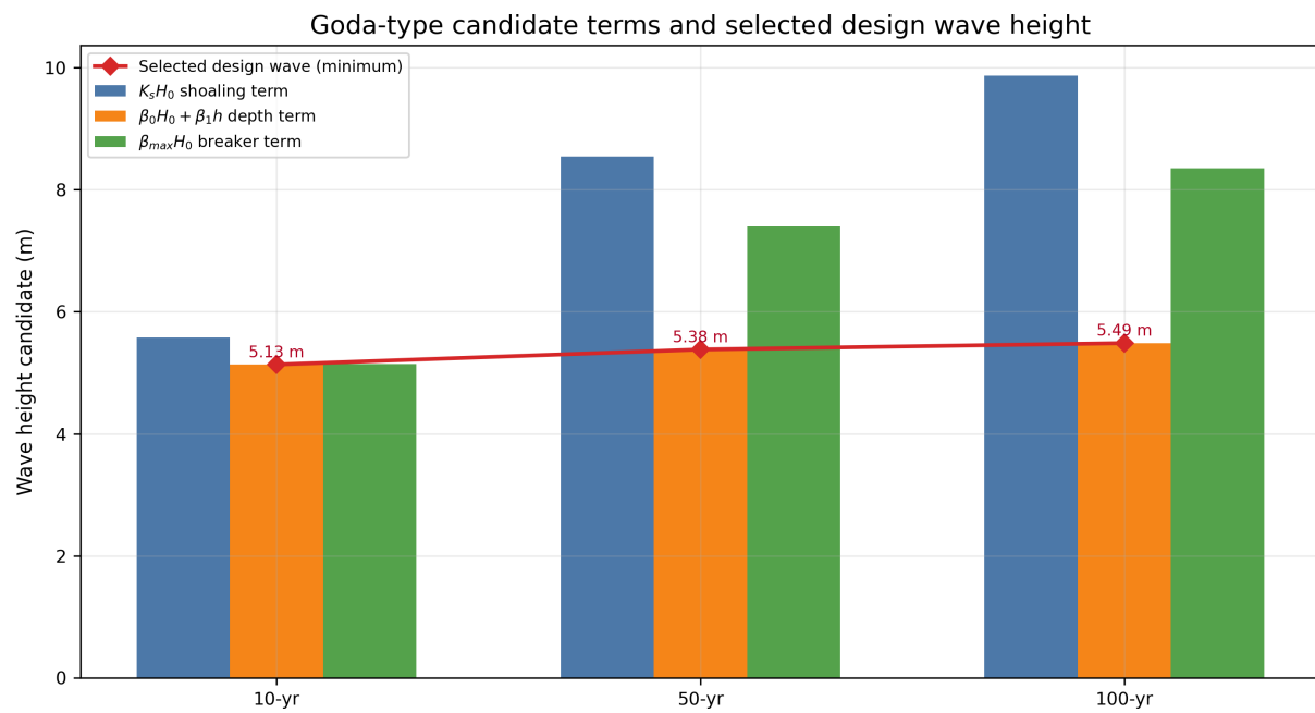
Figure 6: Goda-type candidate terms and selected design wave height.
